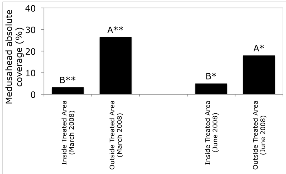
Figure 12. Mean absolute coverage of medusahead in paired observations from precision-grazed plots and areas outside the plots (where livestock had continuous access) at two times during 2008 (the year following precision grazing). Means represented by neighboring columns with different letters are significantly different at the 0.05 or 0.01 level when marked with * or **.
