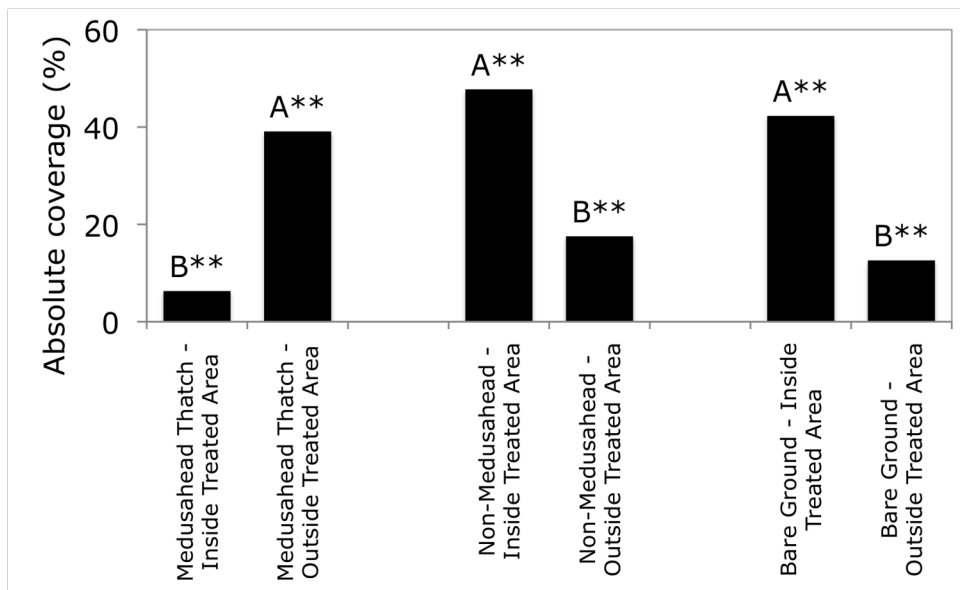
Figure 13. Mean absolute coverage of medusahead thatch, non-medusahead species, and bare ground in paired observations from precision-grazed plots and areas outside the plots (where livestock had continuous access) during March of 2008 (the year following precision grazing).
