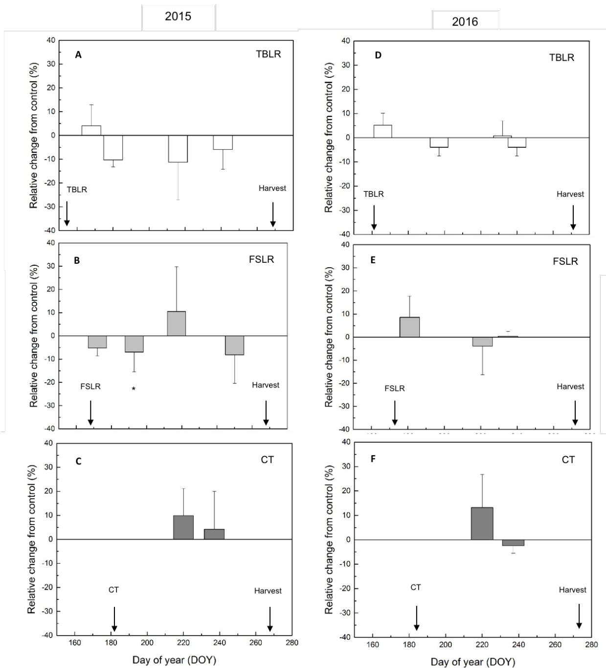
Figure 1. Carbon assimilation rate (A; \mu\text{mol CO}_2 / \text{m}^2 \text{ s} ) expressed as the relative change of the treatment means from the control for trace bloom leaf removal (TBLR; top; A, D), fruit set leaf removal (FSLR; center; B, E), and cluster thinning (CT; bottom; C, F) in 2015 and 2016. Arrows denote dates of treatment application and harvest. In panel B, the asterisk denotes a significant difference between the treatment and control ( P < 0.10 ).
