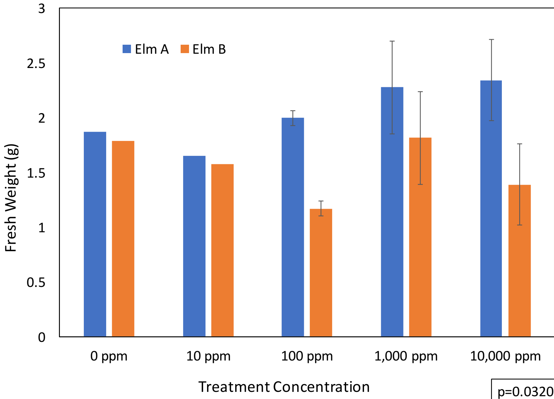
Figure 3b. Hydroponic kale in 50% Hoagland's solution with fungal secretions added at a range of concentrations. Strain is shown within concentration for the strain*concentration interaction.
